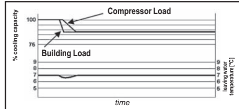
ELWT fluctuation with stepless capacity control
