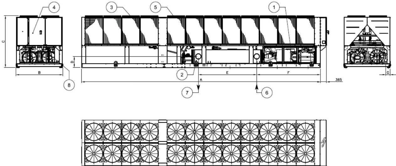
EWAD-C- (3 circuits)
