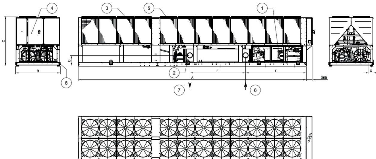
EWAD-C- (3 circuits)
