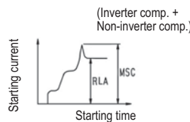
The relationship between the starting time and the starting current
