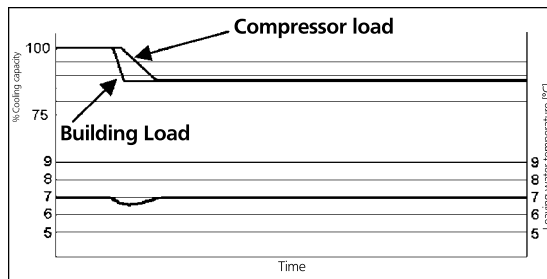
EWLТ fluctuation with stepless capacity control
