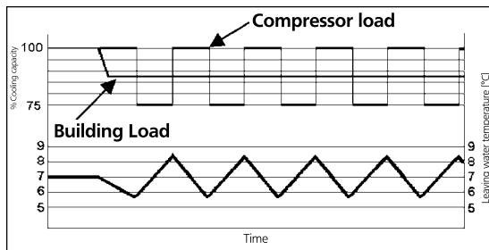
EWLТ fluctuation with steps capacity control (4 steps)
