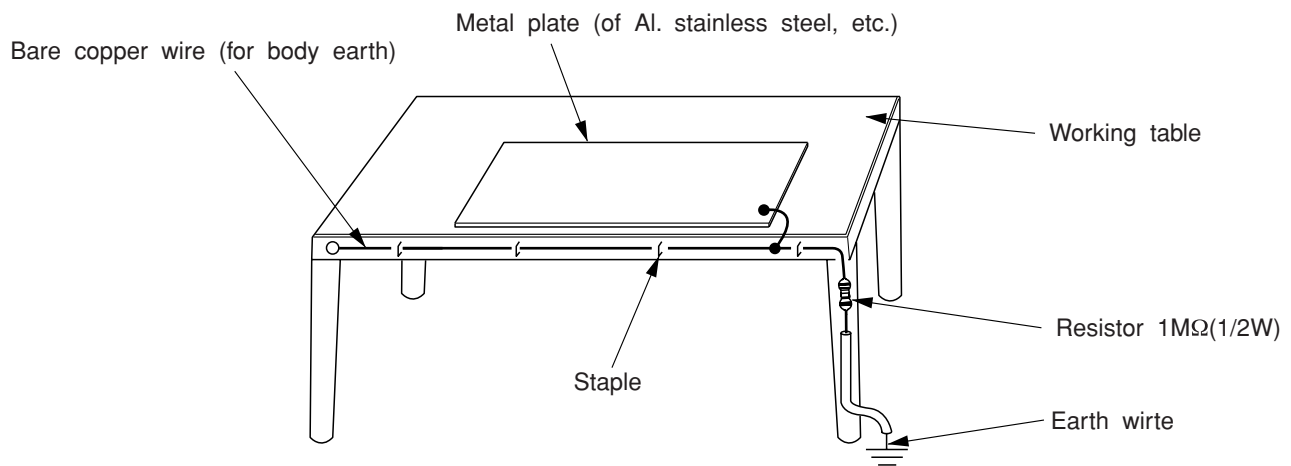
Fig.3 Grounding of the working table
