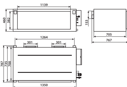
BLC_D/in-100HN1_24Y
