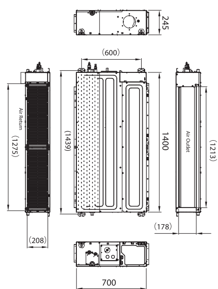
BLC_D/in-48-60HN1_21Y
