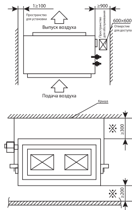
BLC_D/in-80HN1_21Y
