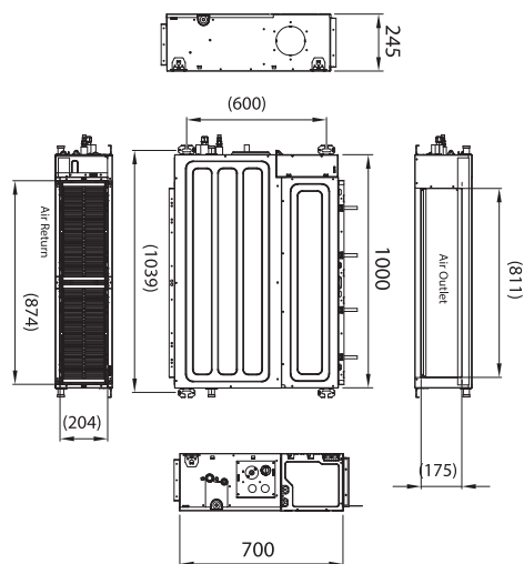
BLC_D/in-48-60HN1_21Y
